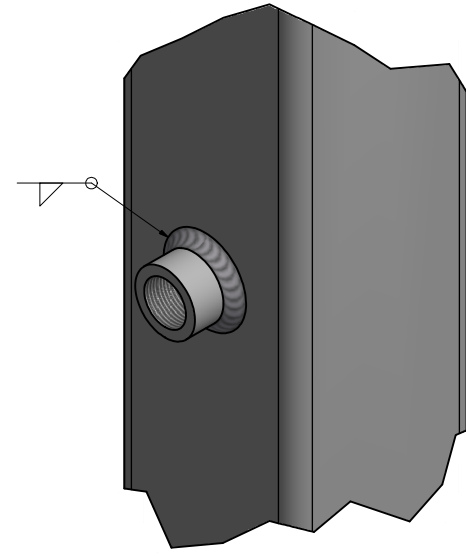
WELDED COUPLING
